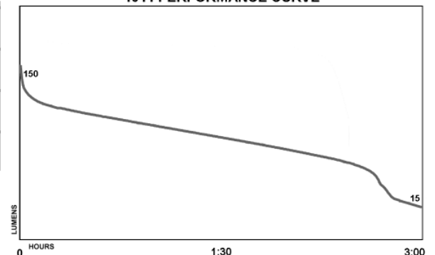
4614 PERFORMANCE CURVE
